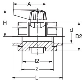
621.342.200 EPDM 621.342.205 FKM (FPM) PVC-U Kugelhahn verschraubt Runddichtring-EPDM grau PVC-U Ball valve with Union-nuts O-Ring-gasket-EPDM grey
