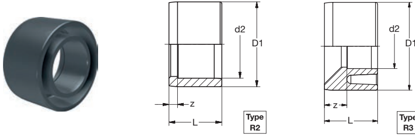
621.90.03 PVC-U Reduktion kurz grau PVC-U Reducer short grey
