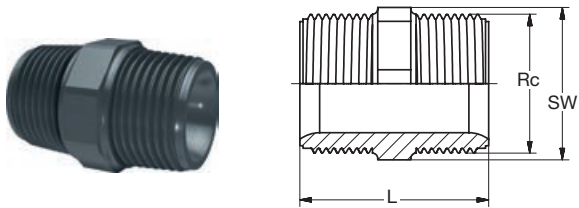
621.91.19 PVC-U Doppelnippel AG-keg grau PVC-U Hexagon nipple male-thread-con grey
