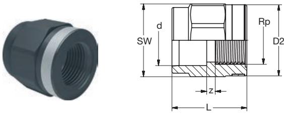
621.91.02 PVC-U Ü-Muffe IG-zyl grau PVC-U Transition-Socket female-thread-cyl grey
