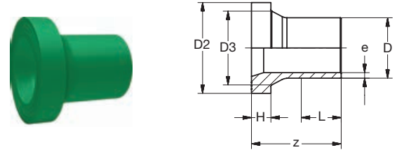
G 8792B PP-RCT V-Bund Klappe gerillt lang st SDR6 grün PP-RCT Flange adaptor valve spigot grooved long butt SDR6 green
