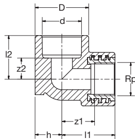
620.100 PVC-U-RG Ü-Winkel 90 IG-zyl Wandbefestigung grau PVC-U-Bronze Transition-Elbow female-thread-cyl wall-mount grey
