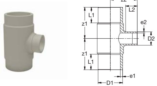
PP-INDUSTRIAL T-Stück 90° red kurz st SDR11 grau PP-INDUSTRIAL Tee 90° red short butt SDR11 grey
