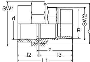
621.54.07 PVC-U-V2A Ü-Verschraubung AG-keg Flachdichtring-EPDM grau PVC-U-Stainless Steel Transition-Union male-thread-con flat-gasket-EPDM grey
