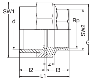
621.54.02 PVC-U-V2A Ü-Verschraubung IG-zyl Flachdichtring-EPDM grau PVC-U-Stainless Steel Transition-Union female-thread-cyl flat-gasket-EPDM grey
