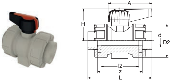
BG 8852 PP-INDUSTRIAL Kugelhahn verschraubt grau PP-INDUSTRIAL Ball valve with union-nuts grey
