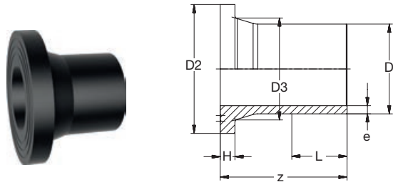
25.80.01.103 PE100 V-Bund lang gerillt SDR11 schwarz PE100 Flange adaptor spigot long grooved SDR11 black
