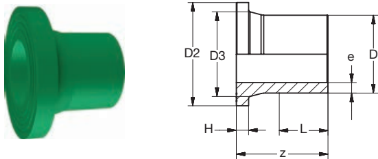
G 8791B PP-RCT V-Bund gerillt lang st SDR11 grün PP-RCT Flange adaptor spigot grooved long butt SDR11 green
