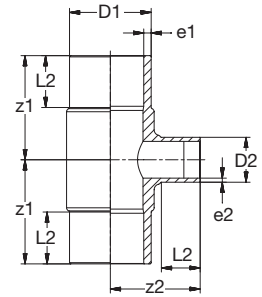
G 8130B PP-RCT T-Stück 90° red lang st SDR11 grün PP-RCT Tee 90° red long butt SDR11 green
